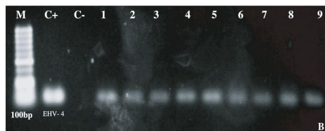
M 100bp DNA ladder. C+ EHV4 positive control strain TH20p. C- Negative control. Lanes 1-9 Real time PCR products.
