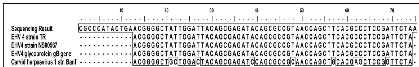
Figure 1. Sequence alignment of the 75 bp amplified fragment of real-time PCR products.
