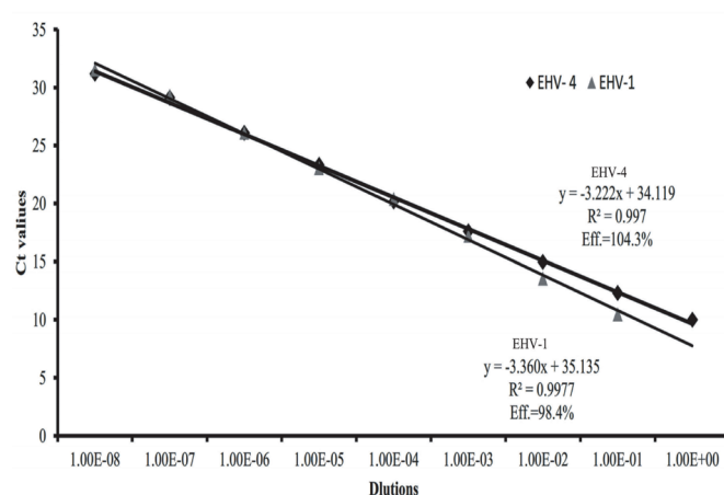
Figure 3. Standard curve of the EHV-1 and EHV-4 real-time PCR assay obtained from triplicates of 10-fold dilutions of standard DNA.
