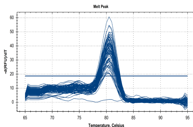
Figure 2. Post-amplification melting curve analysis of EHV-4 positive samples (A)
